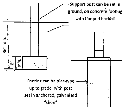
4 Footing Detail
