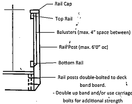
2 Railing Detail Typical detail - many variations available
