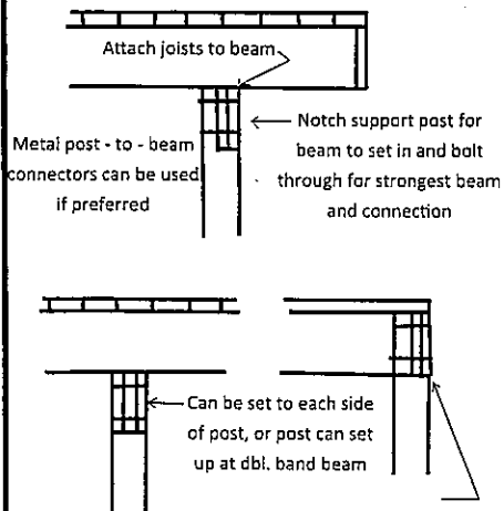
3 Beam / Post Detail
