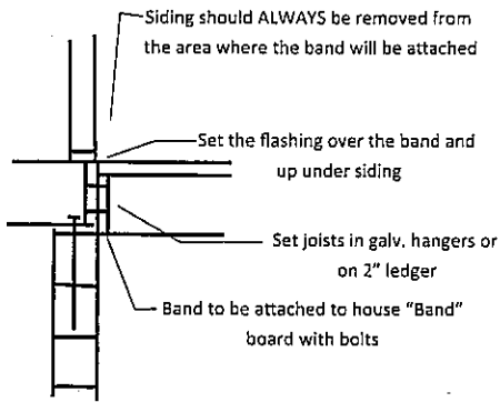
1 Band Detail Shown for frame / siding condition
